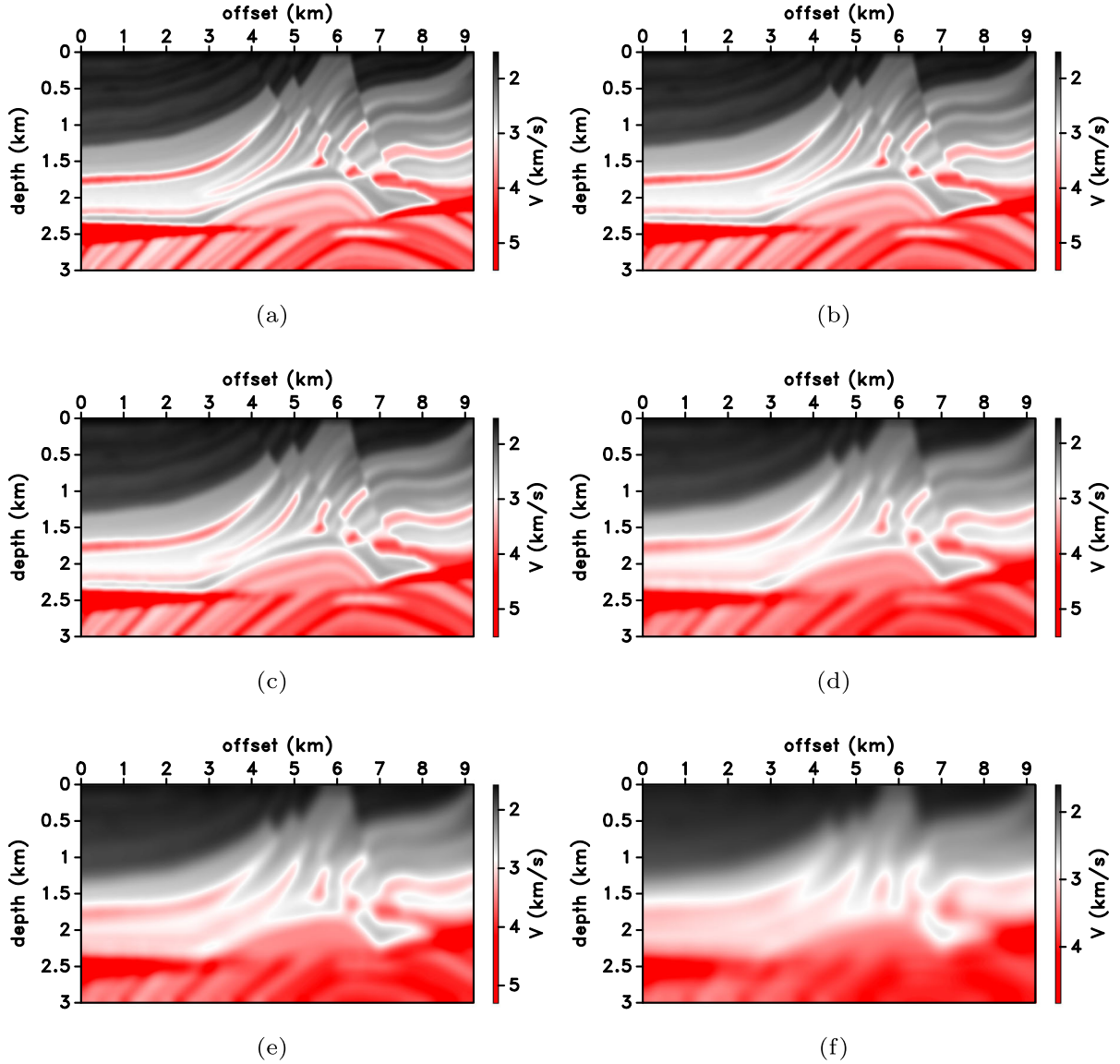
Figure 25 Marmousi velocity model in Fig. 19a after applying smoothing with a radius of 0.08 km, 0.09 km, 0.11 km, 0.16 km, 0.2 km, and 0.3 km, shown in a, b, c, d, e, and f, respectively
