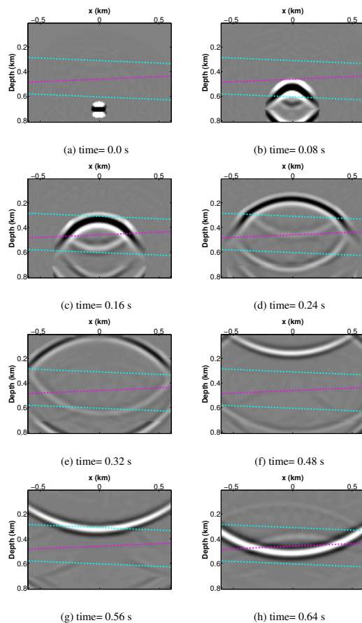
Figure 5: Snapshots of the virtual Green's function G(\mathbf{x}_i', \mathbf{x}_j'', t) with virtual sources \mathbf{x}_j'' = (0, 0.7) km and virtual receivers \mathbf{x}_i' populating the target box in Figure 4a. The dotted lines represent the velocity interface (blue) and the density interface (magenta).
