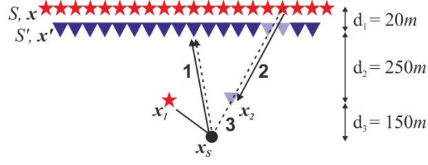
Fig. C-9: Example set of raypaths used in G_S G_0 G_S^* , symbol key as in Fig. C-2 . Rays shown are 1: G_S(\mathbf{x}', \mathbf{x}_1) , 2: G_0(\mathbf{x}_2, \mathbf{x}) , 3: G_S^*(\mathbf{x}', \mathbf{x}) .
