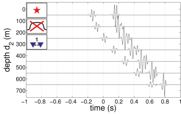
Fig. C-12: G_0G_0G_0^* for different depths \mathbf{d}_2 showing the move-out of non-stationary events.
