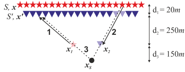
Fig. C-2: Example set of raypaths used in G_0 G_0 G_S^* , symbol key as in Fig. 2 . The dashed line represents the ray of the complex conjugated term. Faded symbols are used to make raypaths visible. Rays shown are 1: G_0(\mathbf{x}', \mathbf{x}_1) , 2: G_0(\mathbf{x}_2, \mathbf{x}) , 3: G_S^*(\mathbf{x}', \mathbf{x}) .
