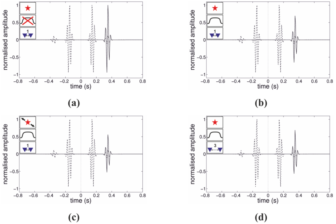
Fig. C-5: Interferometric result of the cross term G_S G_S G_S^* in Eq. (8) (solid line) compared to the true Green's function between \mathbf{x}_1 and \mathbf{x}_2 (dashed line) for different parameter constellations (see Table 2 ). Traces have amplitudes that are normalised relative to case (a).
