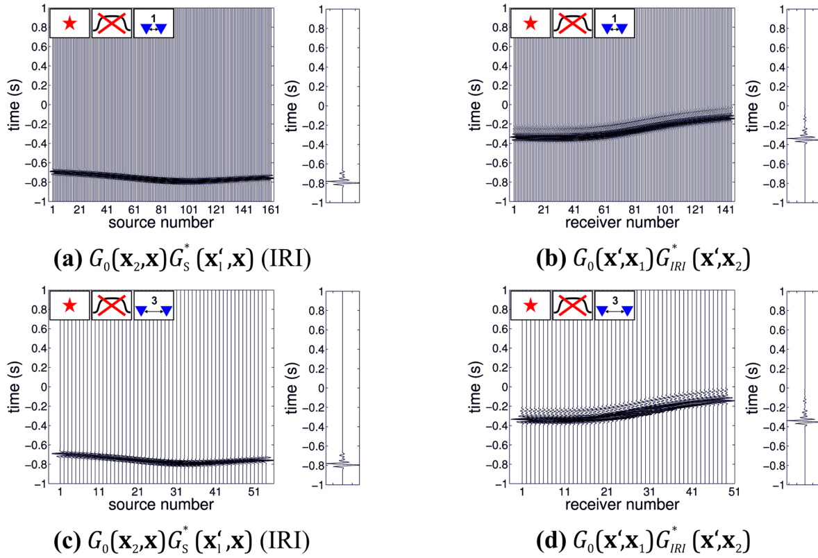
Figure 13. Correlation gathers of G_0 G_0 G_S^* for different parameter constellations (for symbol key see Table 2). Panels (a) and (b) correspond to (a) and (b) in Fig. 10. (c) As in (a) but with the source interval equal to 3 * \lambda_{Nyq} . (d) As in (b) but with the receiver interval equal to 3 * \lambda_{Nyq} . Figure layout as in Fig. 10. In this example the coarser spatial sampling does not affect the interferometric result.
