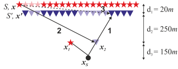
Fig. C-18: Example set of raypaths used in G_S G_0 G_0^* , symbol key as in Fig. C-2 . Rays shown are 1: G_S(\mathbf{x}', \mathbf{x}_1) , 2: G_0(\mathbf{x}_2, \mathbf{x}) , 3: G_0^*(\mathbf{x}', \mathbf{x}) .
