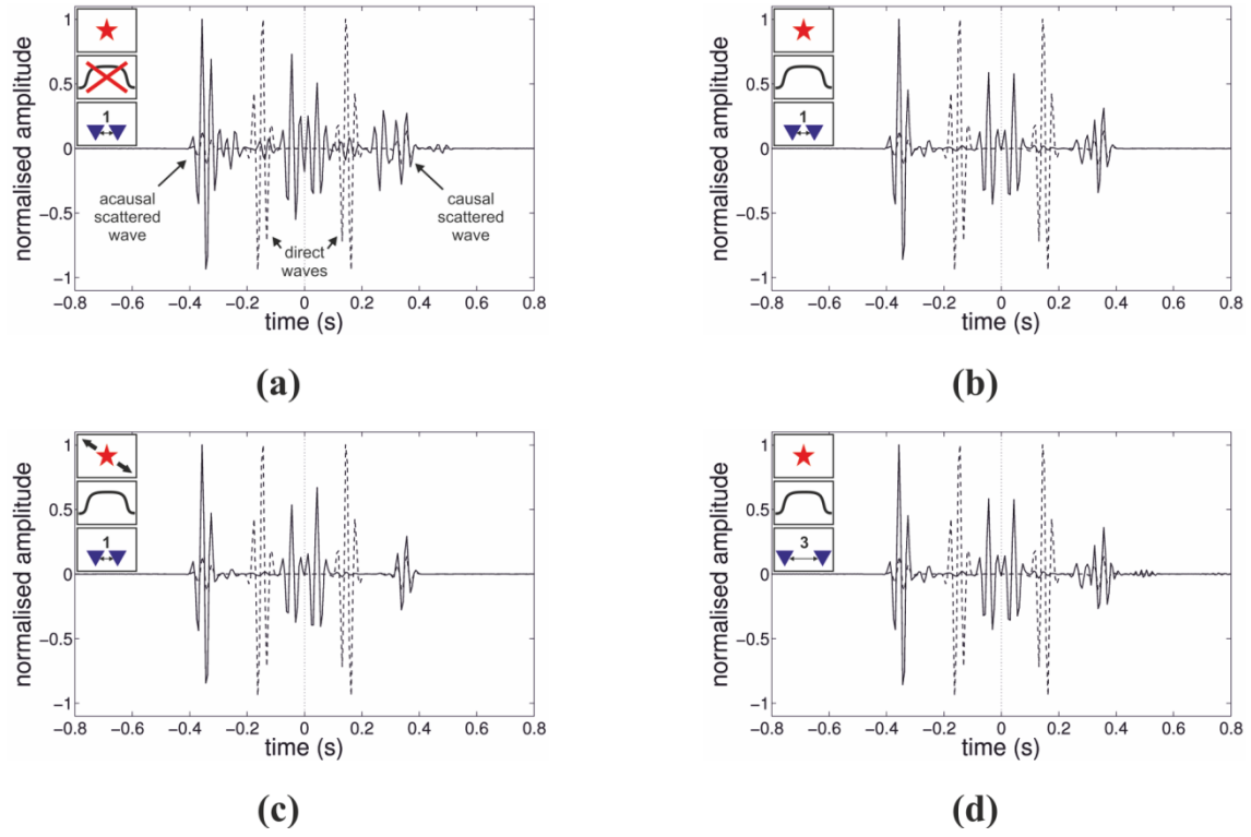
Fig. C-1: Interferometric result of the full integral GGG^* of Eq. (8) (solid line) compared to the true Green's function between \mathbf{x}_1 and \mathbf{x}_2 (dashed line) for different parameter constellations (see Table 2 ). Maximum Amplitudes have been normalised to one.
