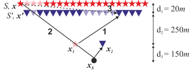
Fig. C-16: Example set of raypaths used in G_0 G_S G_0^* , symbol key as in Fig. C-2 . Rays shown are 1: G_0(\mathbf{x}', \mathbf{x}_1) , 2: G_S(\mathbf{x}_2, \mathbf{x}) , 3: G_0^*(\mathbf{x}', \mathbf{x}) .
