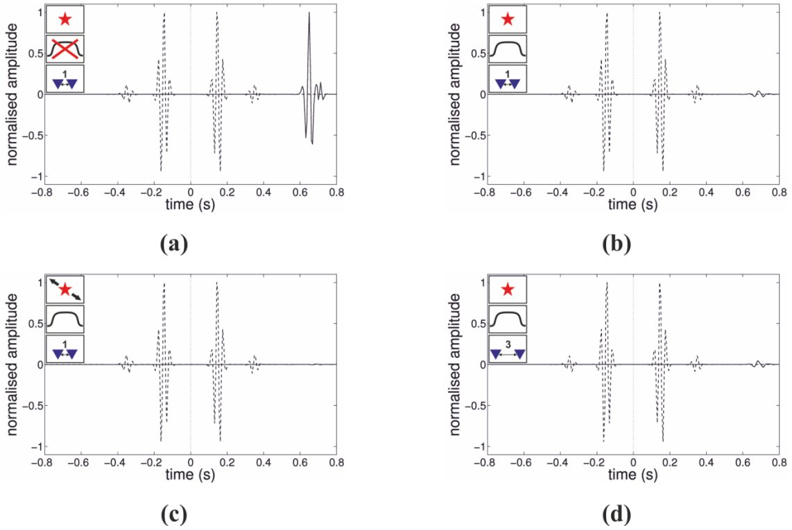
Fig. C-15: Interferometric result of the cross term G_S G_S G_0^* in Eq. (8) (solid line) compared to the true Green's function between \mathbf{x}_1 and \mathbf{x}_2 (dashed line) for different parameter constellations (see Table 2 ). Traces have amplitudes that are normalised relative to case (a).
