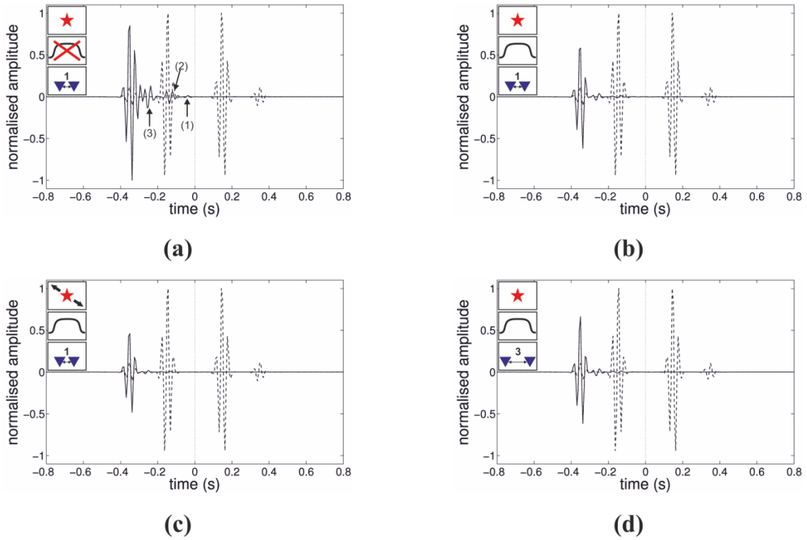
Fig. C-3: Interferometric result of the cross term G_0 G_0 G_S^* in Eq. (8) (solid line) compared to the true Green's function between \mathbf{x}_1 and \mathbf{x}_2 (dashed line) for different parameter constellations (see Table 2 ). Traces have amplitudes that are normalised relative to case (a). Number labels are referred to in the text.
