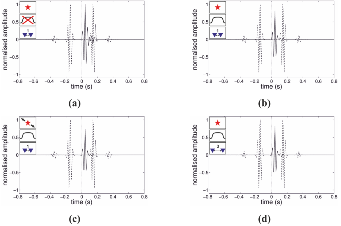
Fig. C-10: Interferometric result of the cross term G_S G_0 G_S^* in Eq. (8) (solid line) compared to the true Green's function between \mathbf{x}_1 and \mathbf{x}_2 (dashed line) for different parameter constellations (see Table 2 ). Traces have amplitudes that are normalised relative to case (a).
