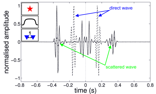
Figure 8. Source–receiver interferometric estimate of the Green's function between \mathbf{x}_1 and \mathbf{x}_2 using the full wavefield and the incomplete boundaries in Fig. 7 (solid line), compared to the true Green's function (dashed line). Amplitudes of each waveform have normalized maximum values. For legend key see Table 2.
