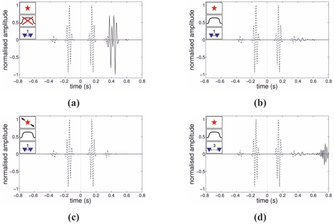
Fig. C-19: Interferometric result of the cross term G_S G_0 G_0^* in Eq. (8) (solid line) compared to the true Green's function between \mathbf{x}_1 and \mathbf{x}_2 (dashed line) for different parameter constellations (see Table 2 ). Traces have amplitudes that are normalised relative to case (a). Inset in (d) shows detail.
