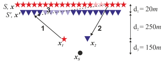
Fig. C-11: Example set of raypaths used in G_0G_0G_0^* , symbol key as in Fig. C-2 . Rays shown are 1: G_0(\mathbf{x}', \mathbf{x}_1) , 2: G_0(\mathbf{x}_2, \mathbf{x}) , 3: G_0^*(\mathbf{x}', \mathbf{x}) .
