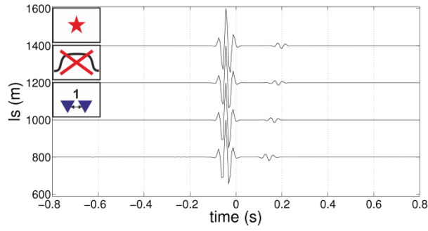
Fig. C-7: G_0 G_S G_S^* for different apertures (length ls ) of both source ( ls ) and receiver ( ls - 100 ) boundary showing a stationary ( -0.05 s) and a non-stationary (between 0.1 and 0.2 s) non-physical arrival.
