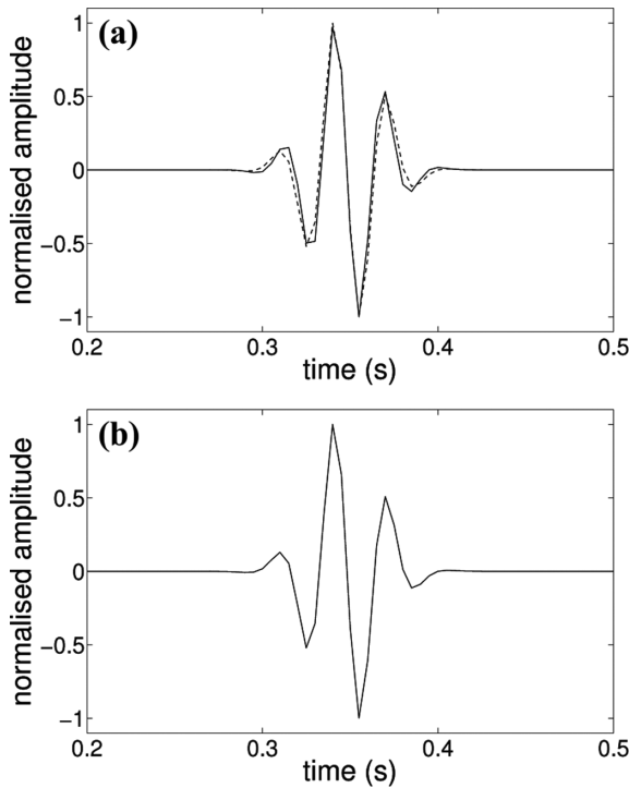
Figure 6. (a) Interferometric result of the term G_S G_S G_S^* in eq. (8) (solid line) compared to the modelled causal scattered wave G_S(\mathbf{x}_2, \mathbf{x}_1) (dashed line) using 3-D Green's functions and the geometry shown in Fig. 7. Amplitudes have been normalized with respect to the maximum of each trace. (b) As in (a) but divided by the wavenumber k in the frequency domain (cf. eq. (14)): the waveforms of the two curves are now identical.
