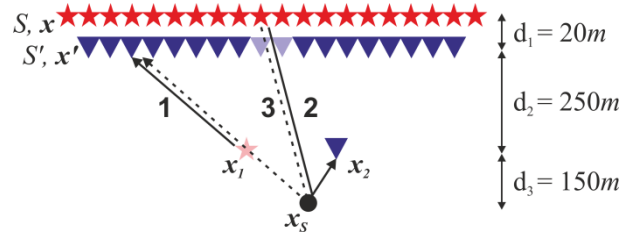
Fig. C-6: Example set of raypaths used in G_0 G_S G_S^* , symbol key as in Fig. C-2 . Rays shown are 1: G_0(\mathbf{x}', \mathbf{x}_1) , 2: G_S(\mathbf{x}_2, \mathbf{x}) , 3: G_S^*(\mathbf{x}', \mathbf{x}) .
